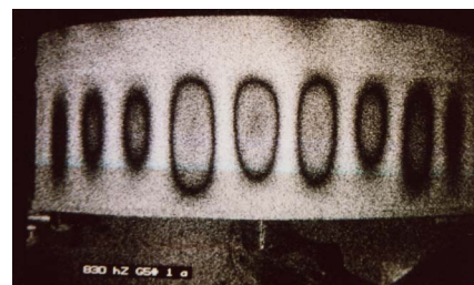
Figure 8: Mode coupling in G_5 (small right bottom), G_4 (lower left), and C_4 (upper left) note sections
