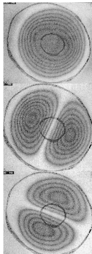
Figure 12: Ping C_4 note section Modes (0,0) 262.2 Hz, (0,1) 519.2 Hz, and (1,0) 773.4 Hz.
