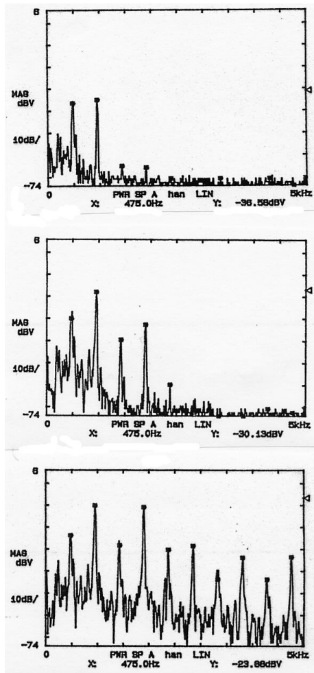
Figure 2: Sound spectra of A_4^\# note section of PanArt lead Tenor Pan with mallet blow near the front of the section top: soft-; middle: medium-; bottom: hard blow
