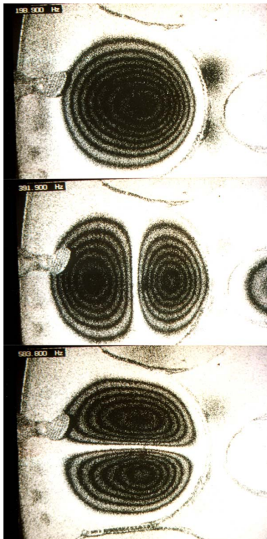
Figure 5: The lowest three partials of a G_3 note sections at 198.9 Hz, 391.9 Hz, and 583.8 Hz (from top to bottom)
