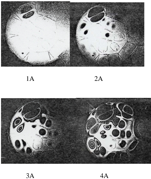
Figure 10: Second mode of a D 4 note section of a double second pan, driven with increasing amplitude.
