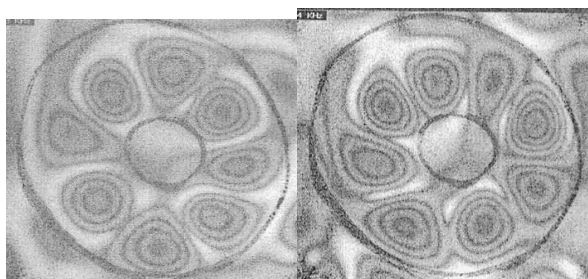
Figure 14: Two higher modes of a C_4 ping note section Left 3725 Hz, right 3904 Hz
