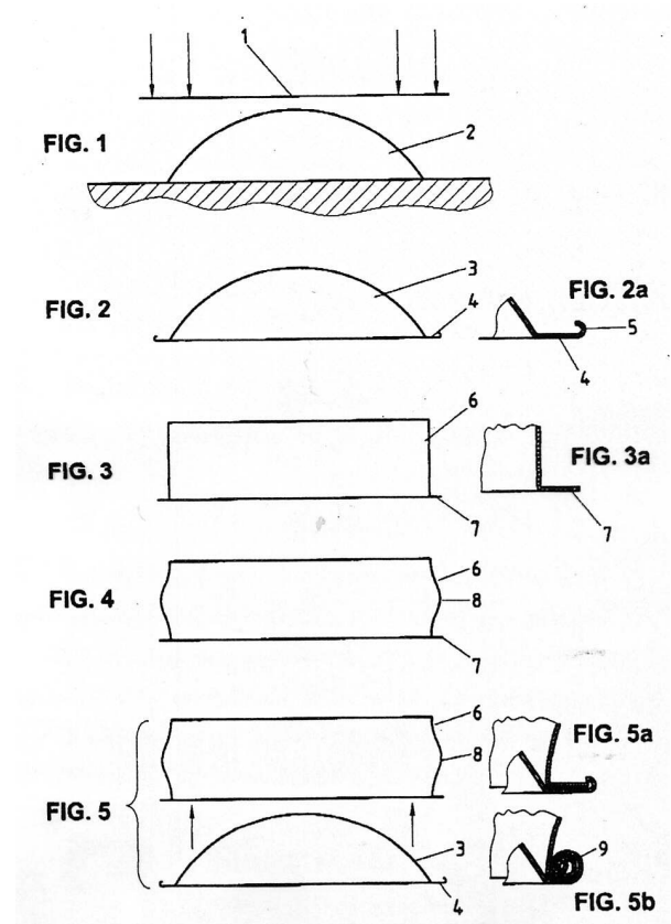
Figure 11: Steps in mechanical pan preparation (courtesy Felix Rohner of PanArt)
