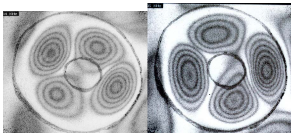
Figure 13: Two (1,1) modes of a C_4 ping note section Left 2004 Hz; right 2066 Hz
