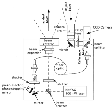
Figure 4: Instrumentation for electronic holographic interferometry.
